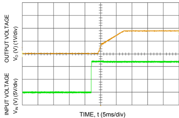
Figure 15. Typical Start-up Using Input Voltage ( V_{IN} = V_{IN,NOM} , I_o = I_{o,max} ).
