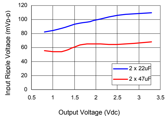
Figure 47. Input ripple voltage in mV, p-p for various output voltages with 2 \times 22\mu F or 2 \times 47\mu F ceramic capacitors at the input (30A load). Input voltage is 5V.
