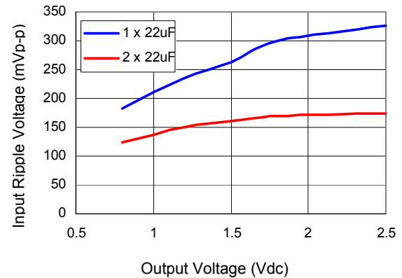
Figure 46. Input ripple voltage for various output voltages with 1 \times 22\mu F or 2 \times 22\mu F ceramic capacitors at the input (30A load). Input voltage is 12V.
